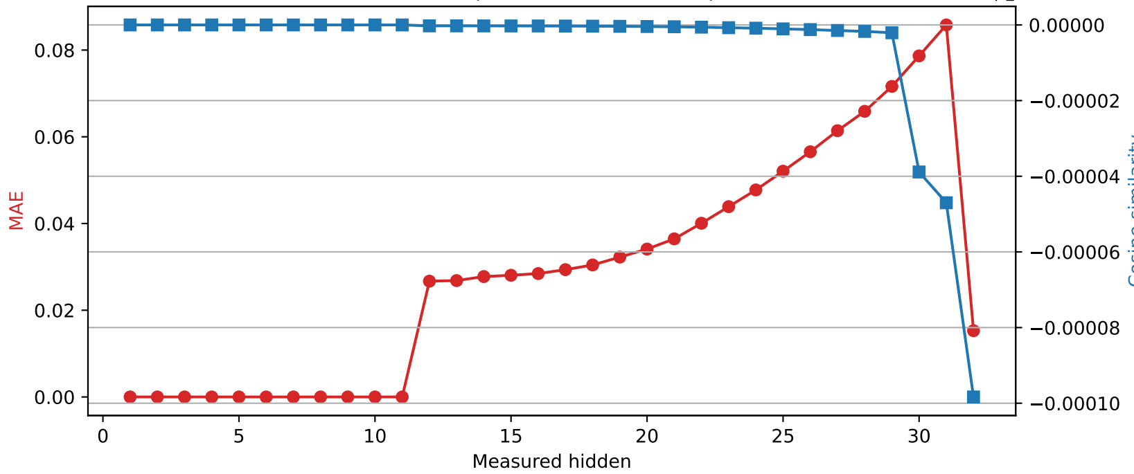
Phi-3-mini-4k-instruct | Quantized layer 11 | float16 \rightarrow int8
