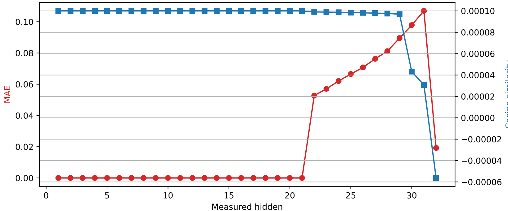
Phi-3-mini-4k-instruct | Quantized layer 21 | float16 → int8
