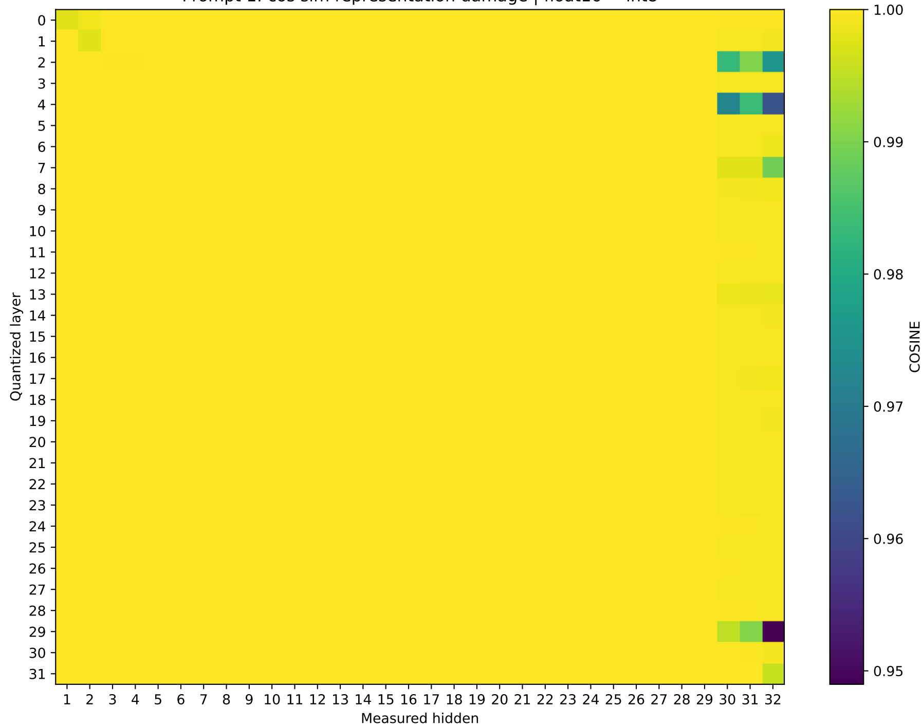
Phi-3-mini-4k-instruct Prompt 1: cos sim representation damage | float16 \rightarrow int8
