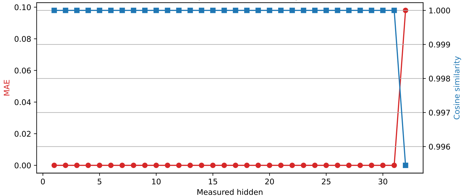
Phi-3-mini-4k-instruct | Quantized layer 31 | float16 \rightarrow int8
