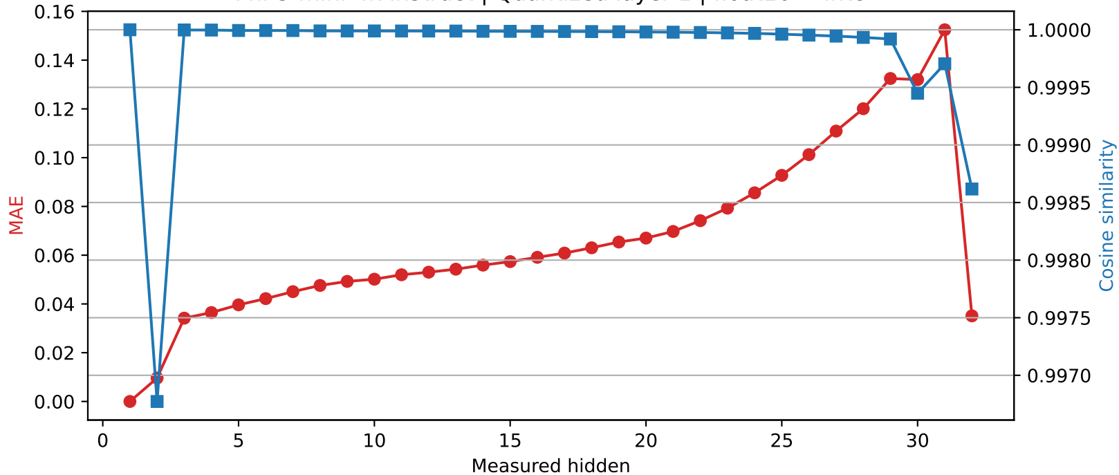
Phi-3-mini-4k-instruct | Quantized layer 1 | float16 \rightarrow int8
