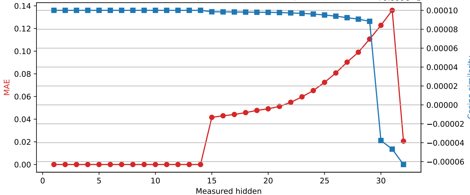
Phi-3-mini-4k-instruct | Quantized layer 14 | float16 → int8
