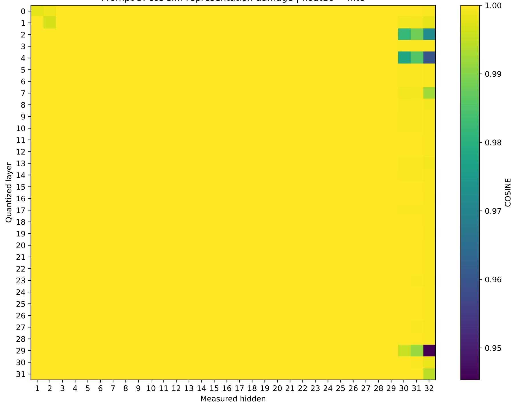
Phi-3-mini-4k-instruct Prompt 3: cos sim representation damage | float16 \rightarrow int8
