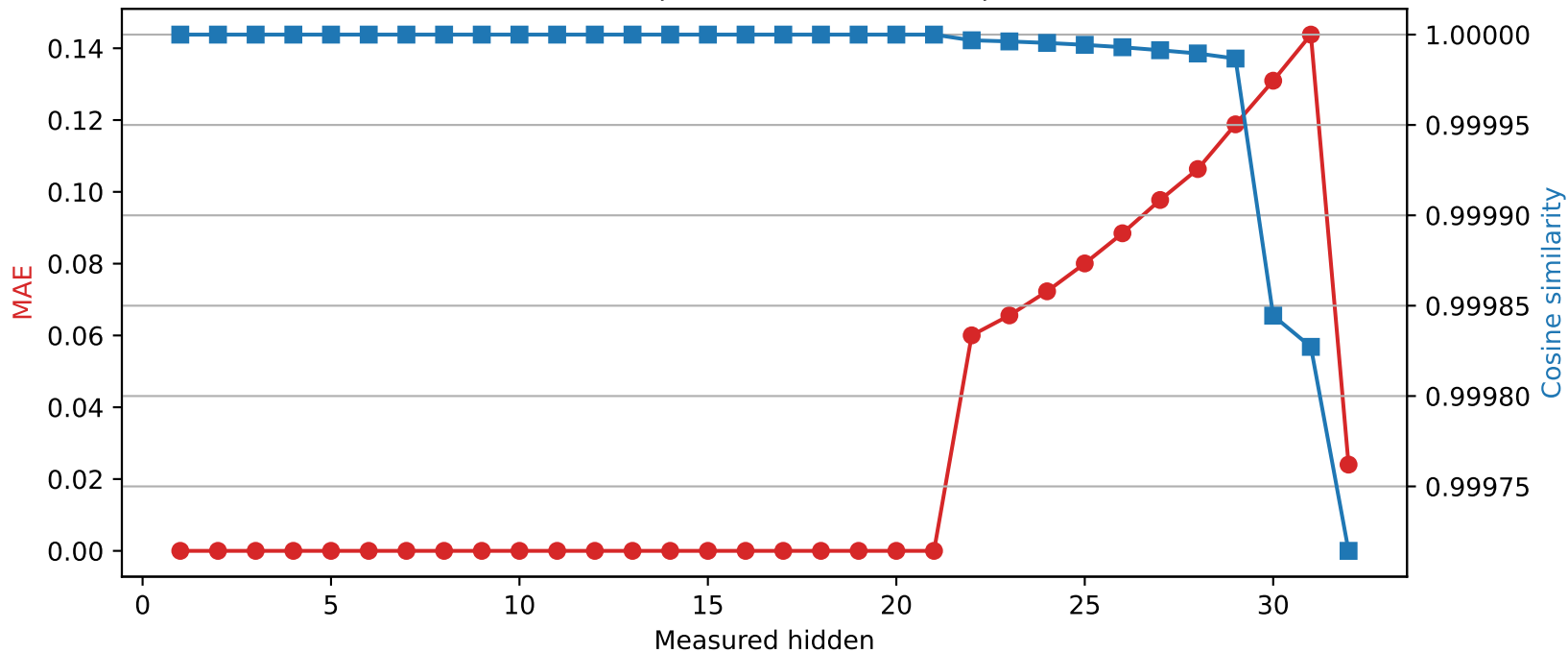
Phi-3-mini-4k-instruct | Quantized layer 21 | float16 \rightarrow int8
