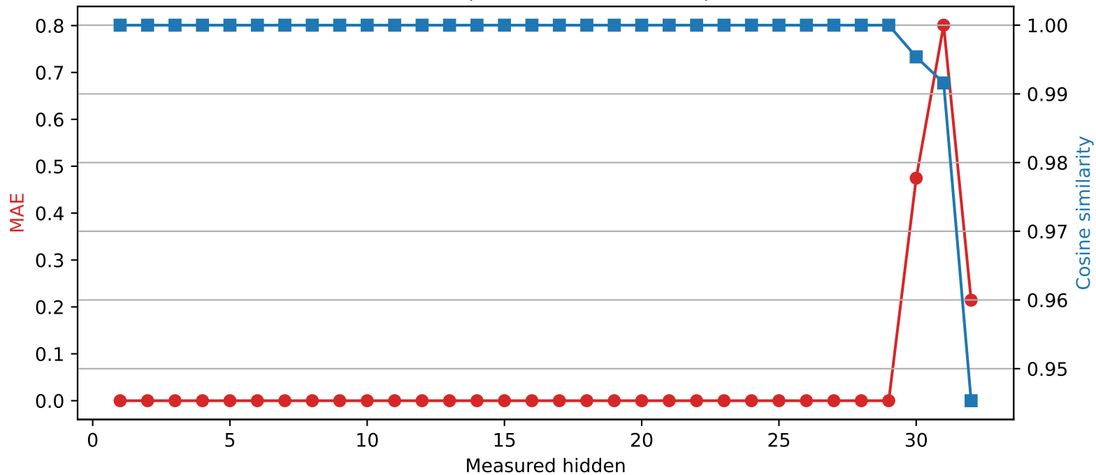
Phi-3-mini-4k-instruct | Quantized layer 29 | float16 \rightarrow int8
