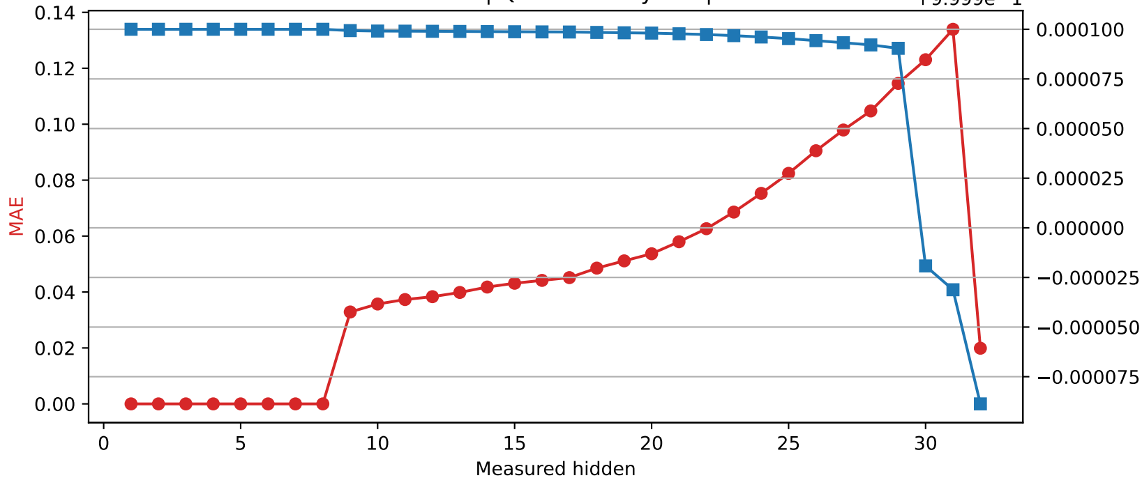
Phi-3-mini-4k-instruct | Quantized layer 8 | float16 → int8
