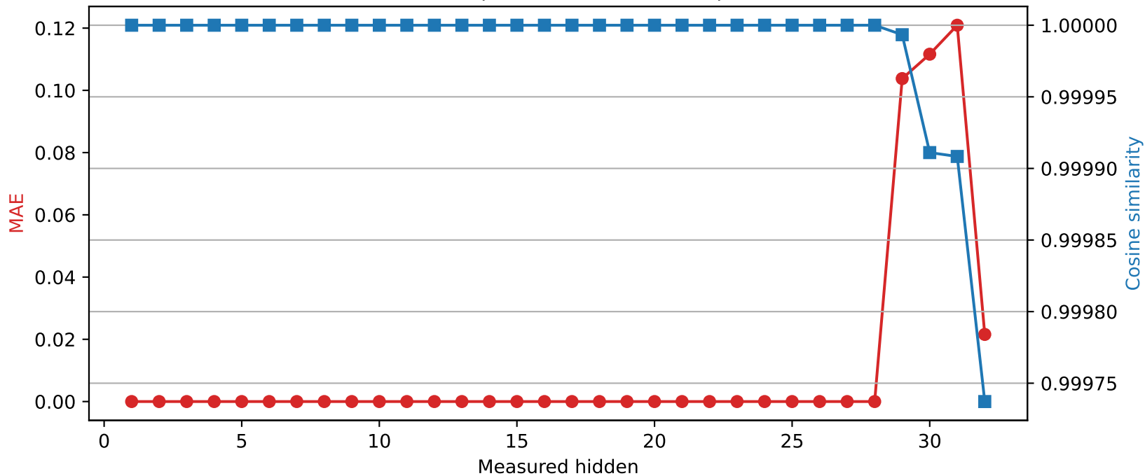
Phi-3-mini-4k-instruct | Quantized layer 28 | float16 \rightarrow int8
