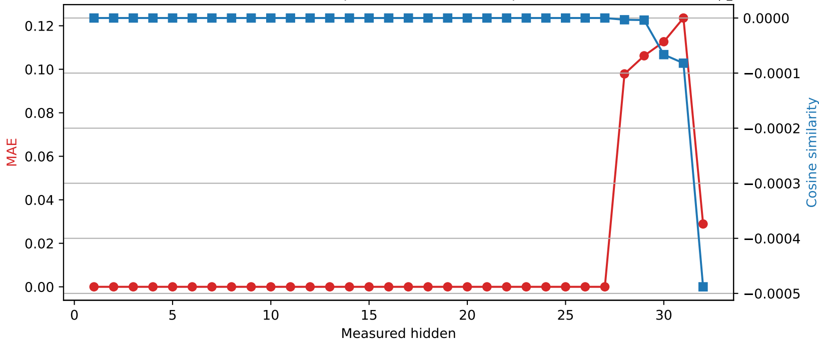
Phi-3-mini-4k-instruct | Quantized layer 27 | float32 \rightarrow int8
