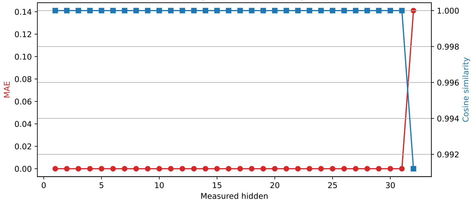
Phi-3-mini-4k-instruct | Quantized layer 31 | float32 \rightarrow int8
