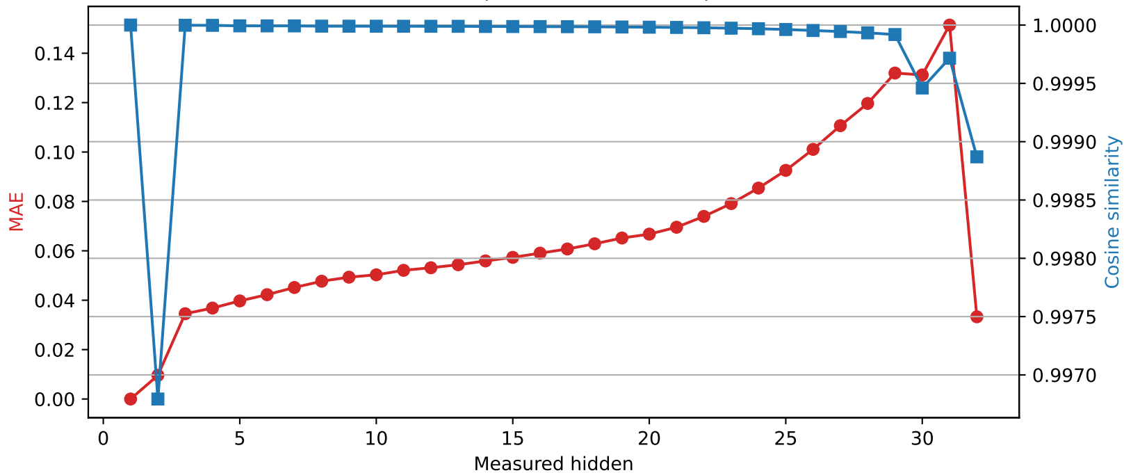
Phi-3-mini-4k-instruct | Quantized layer 1 | float32 \rightarrow int8
