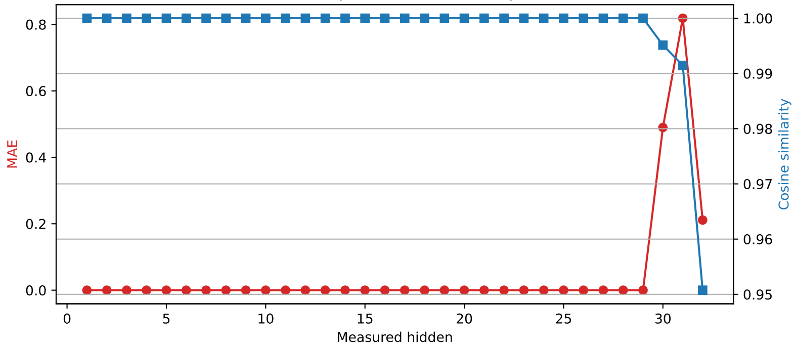
Phi-3-mini-4k-instruct | Quantized layer 29 | float32 \rightarrow int8
