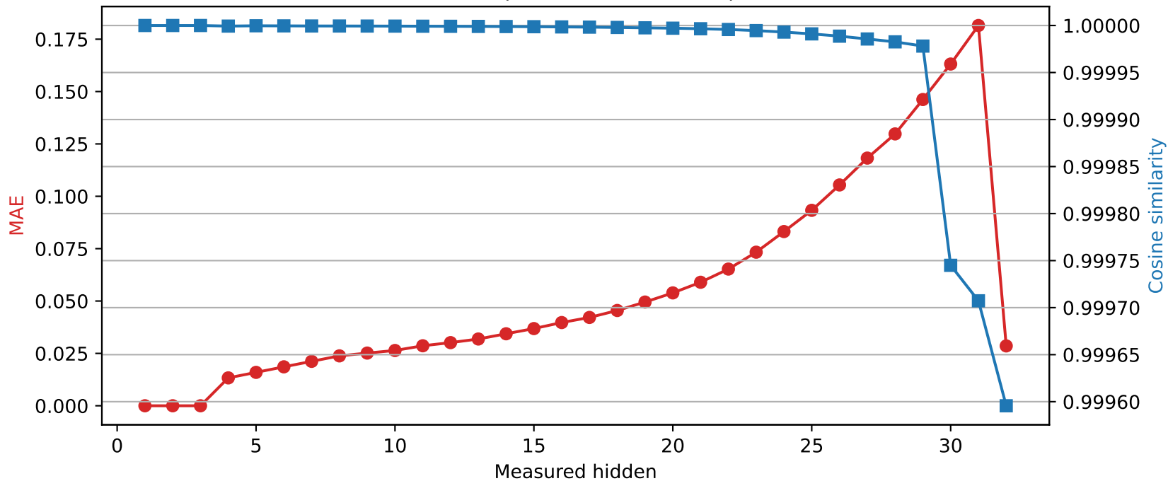
Phi-3-mini-4k-instruct | Quantized layer 3 | float32 → int8
