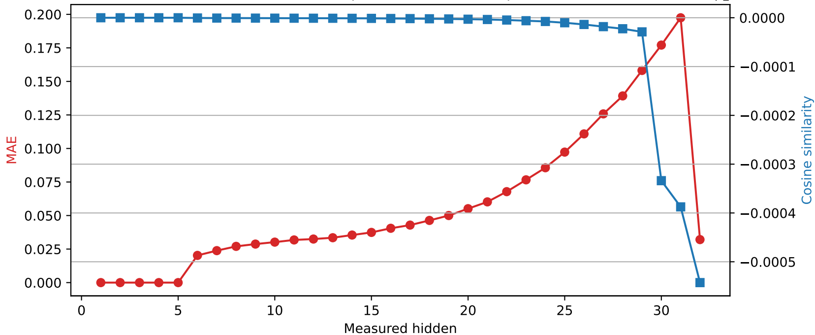
Phi-3-mini-4k-instruct | Quantized layer 5 | float32 → int8
