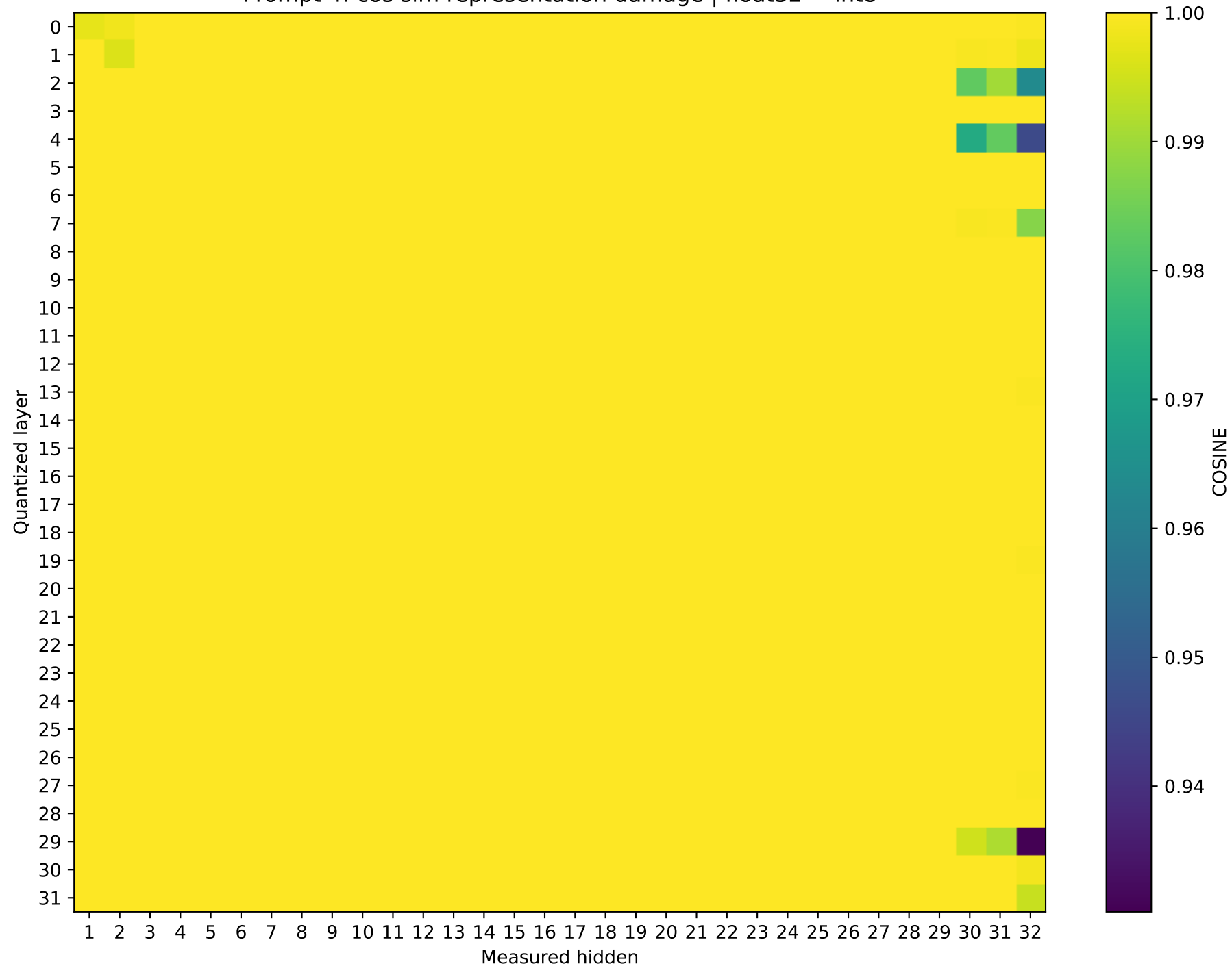
Phi-3-mini-4k-instruct Prompt 4: cos sim representation damage | float32 → int8
