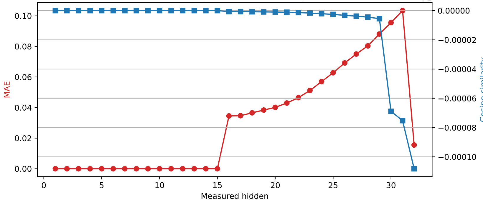
Phi-3-mini-4k-instruct | Quantized layer 15 | float32 → int8
