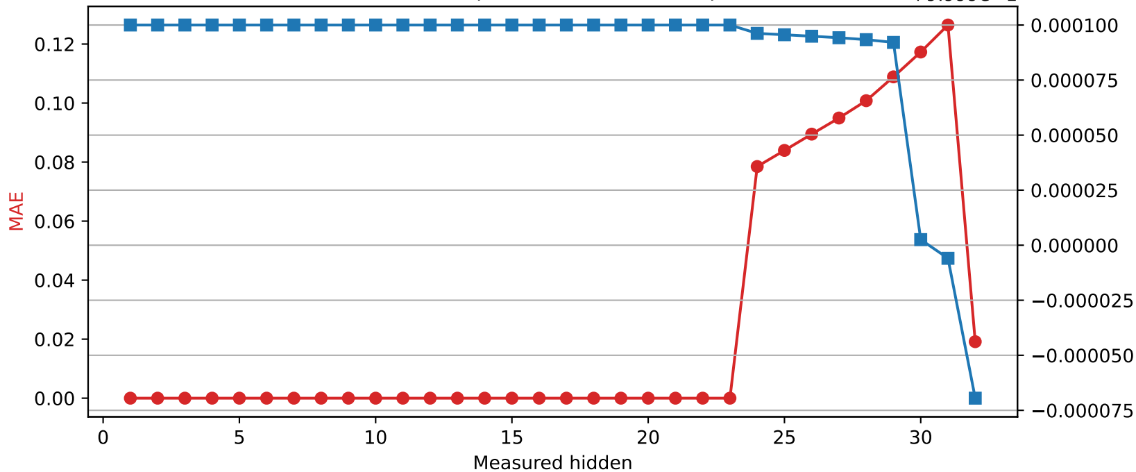
Phi-3-mini-4k-instruct | Quantized layer 23 | float32 → int8
