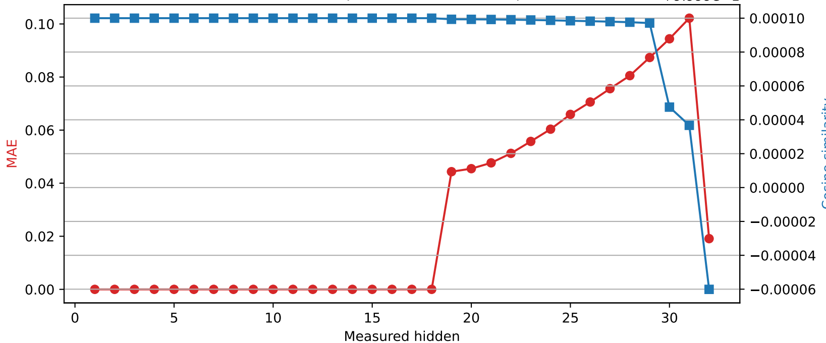
Phi-3-mini-4k-instruct | Quantized layer 18 | float64 \rightarrow int8
