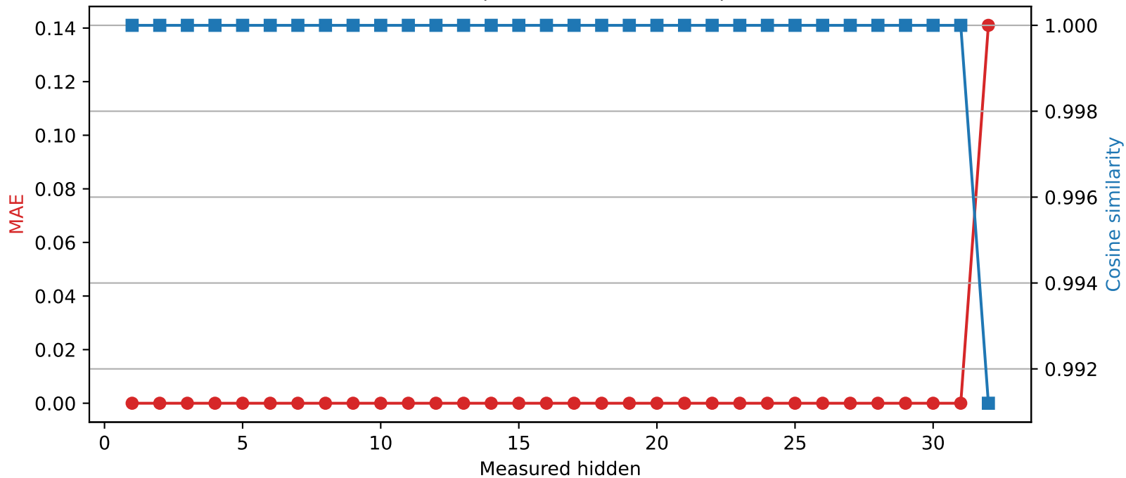
Phi-3-mini-4k-instruct | Quantized layer 31 | float64 \rightarrow int8
