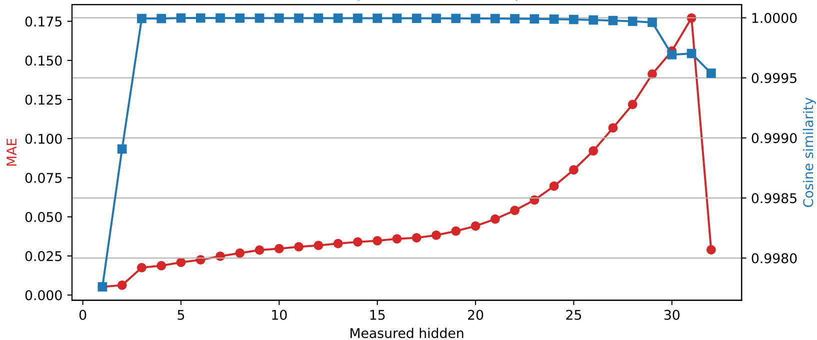
Phi-3-mini-4k-instruct | Quantized layer 0 | float64 \rightarrow int8
