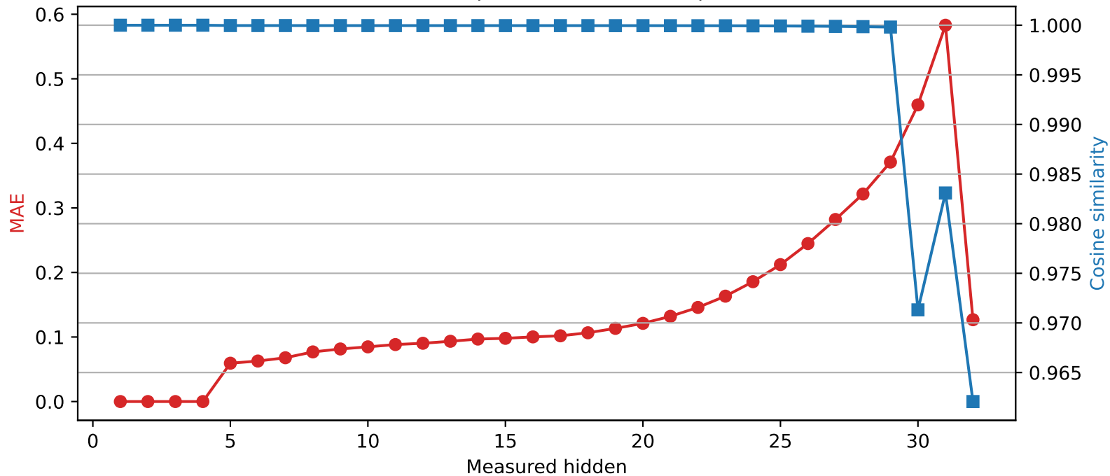
Phi-3-mini-4k-instruct | Quantized layer 4 | float64 → int8
