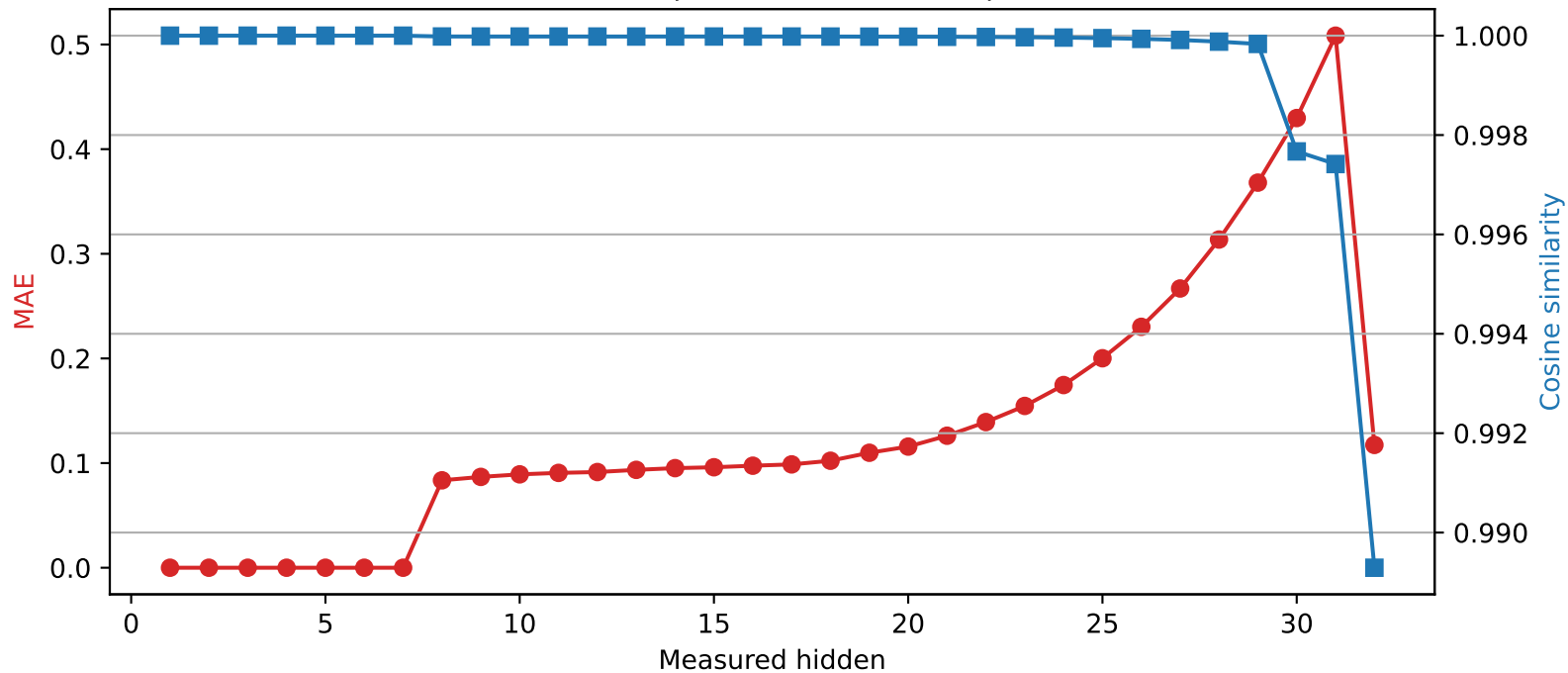
Phi-3-mini-4k-instruct | Quantized layer 7 | float64 \rightarrow int8
