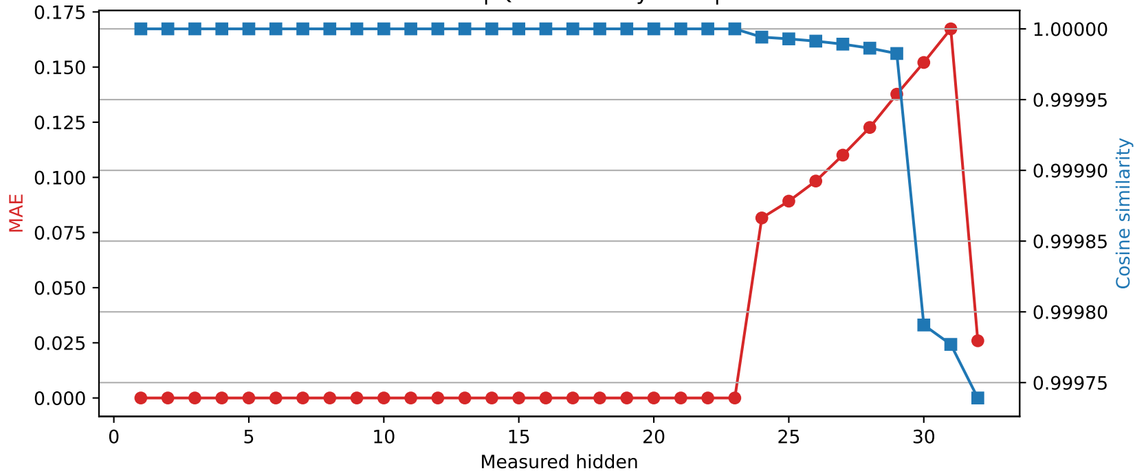
Phi-3-mini-4k-instruct | Quantized layer 23 | float64 → int8
