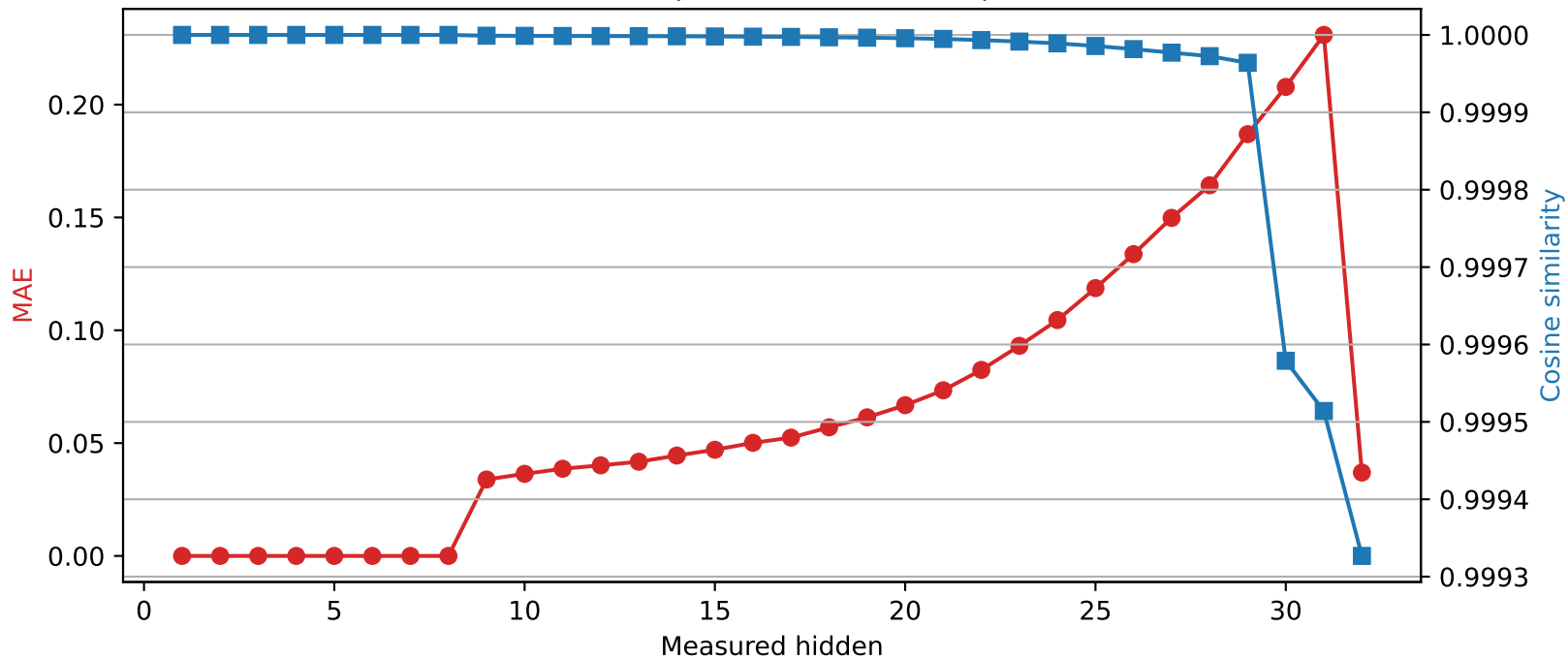
Phi-3-mini-4k-instruct | Quantized layer 8 | float64 → int8
