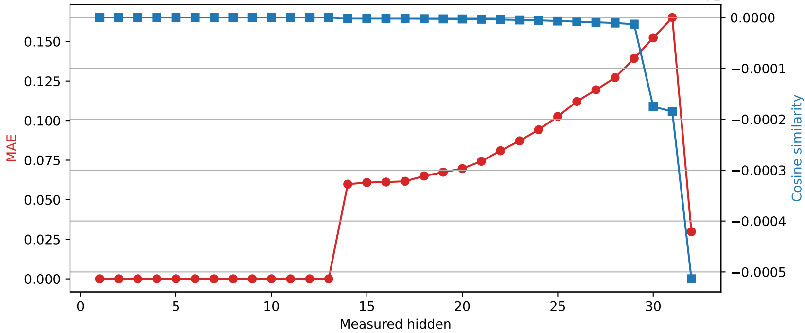
Phi-3-mini-4k-instruct | Quantized layer 13 | float64 → int8
