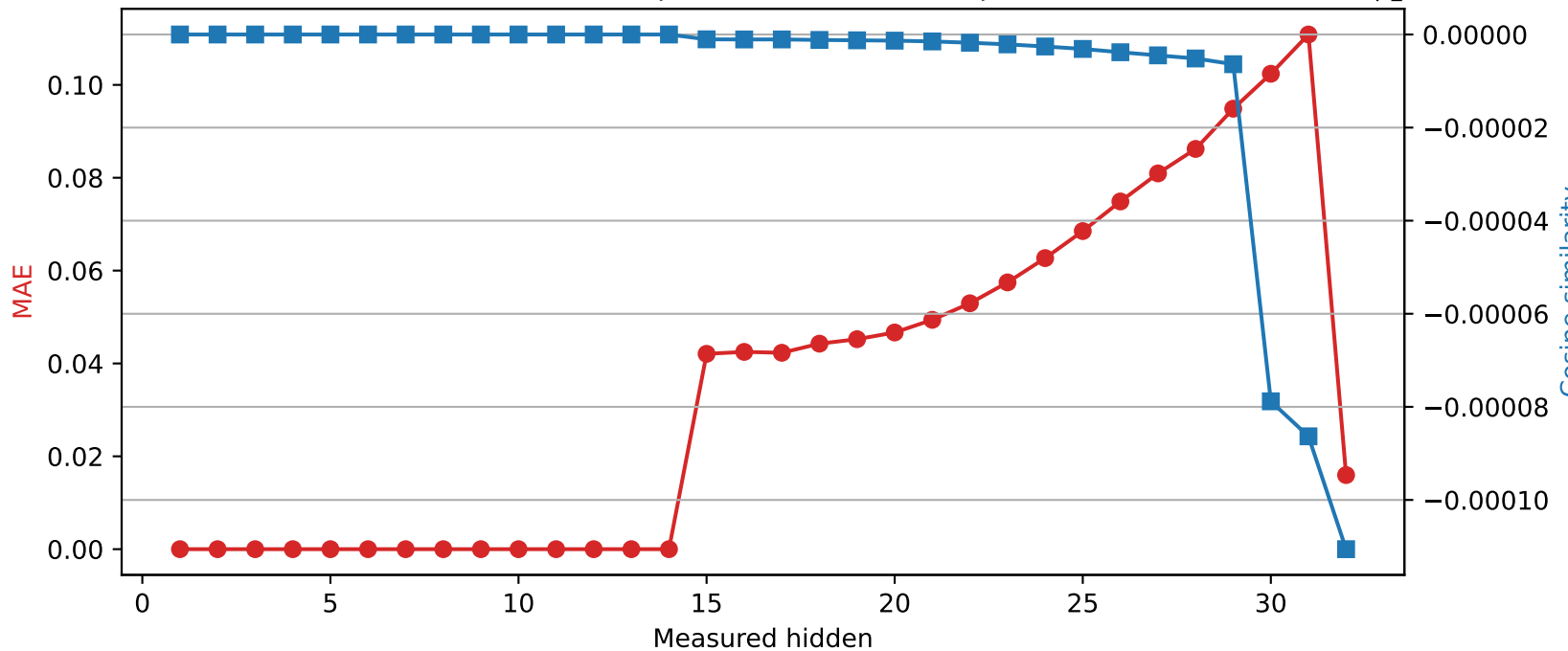
Phi-3-mini-4k-instruct | Quantized layer 14 | float64 → int8
