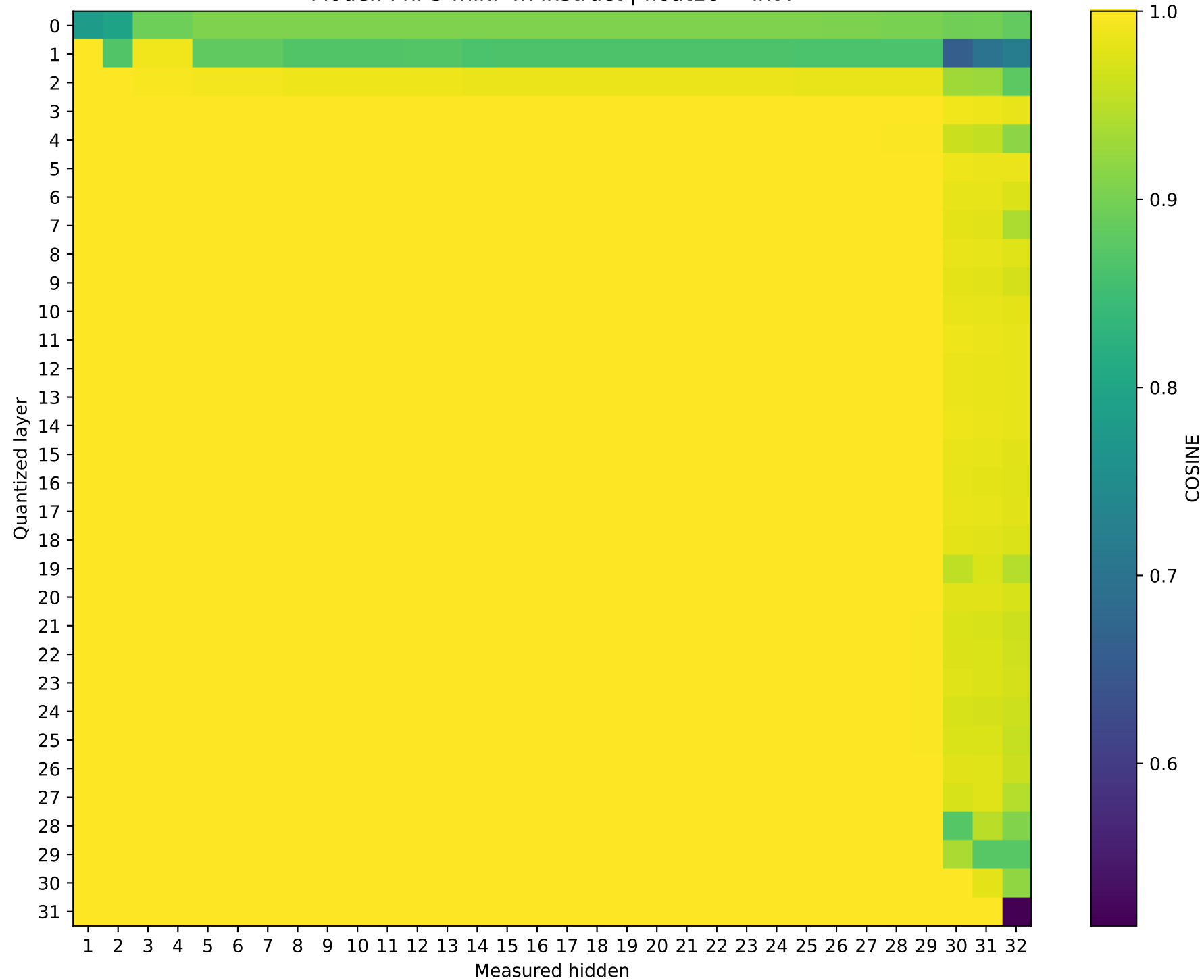
Model: Phi-3-mini-4k-instruct | float16 → int4
