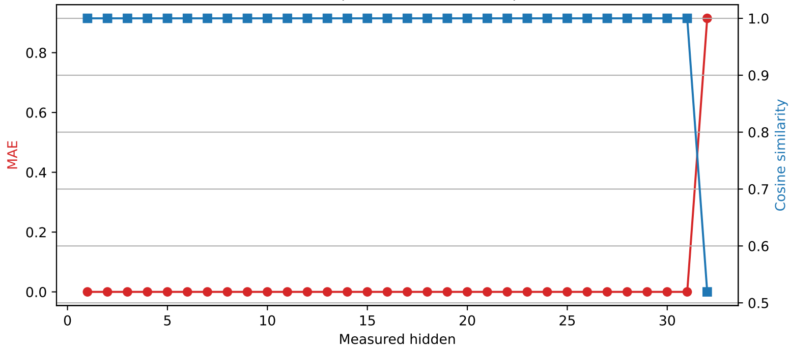
Phi-3-mini-4k-instruct | Quantized layer 31 | float16 \rightarrow int4
