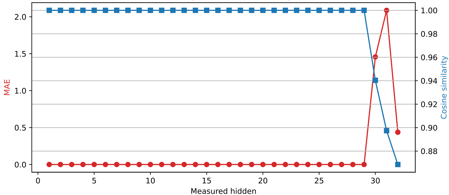
Phi-3-mini-4k-instruct | Quantized layer 29 | float16 \rightarrow int4
