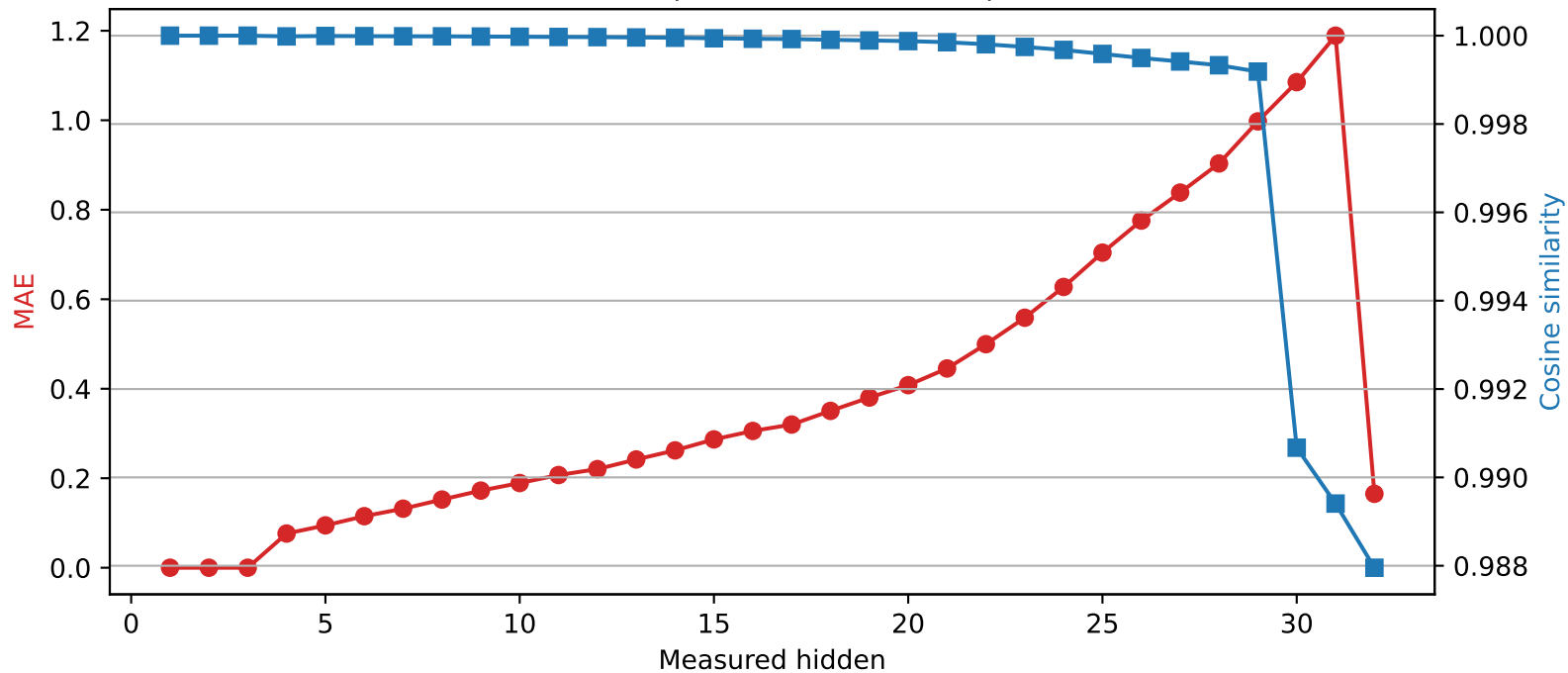
Phi-3-mini-4k-instruct | Quantized layer 3 | float16 \rightarrow int4
