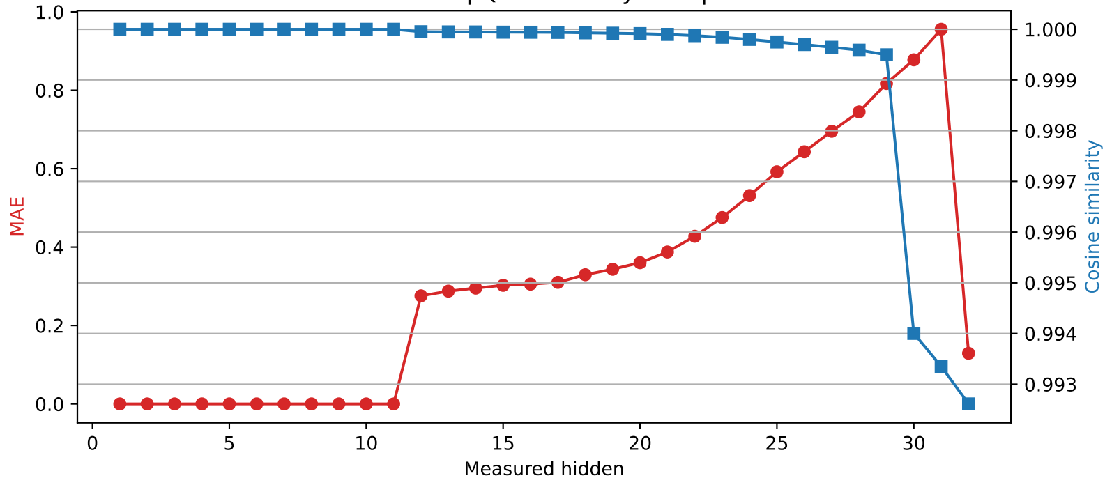
Phi-3-mini-4k-instruct | Quantized layer 11 | float16 \rightarrow int4
