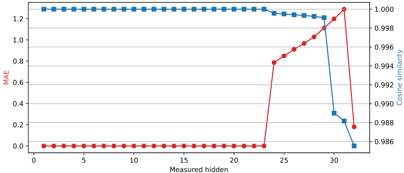
Phi-3-mini-4k-instruct | Quantized layer 23 | float16 \rightarrow int4
