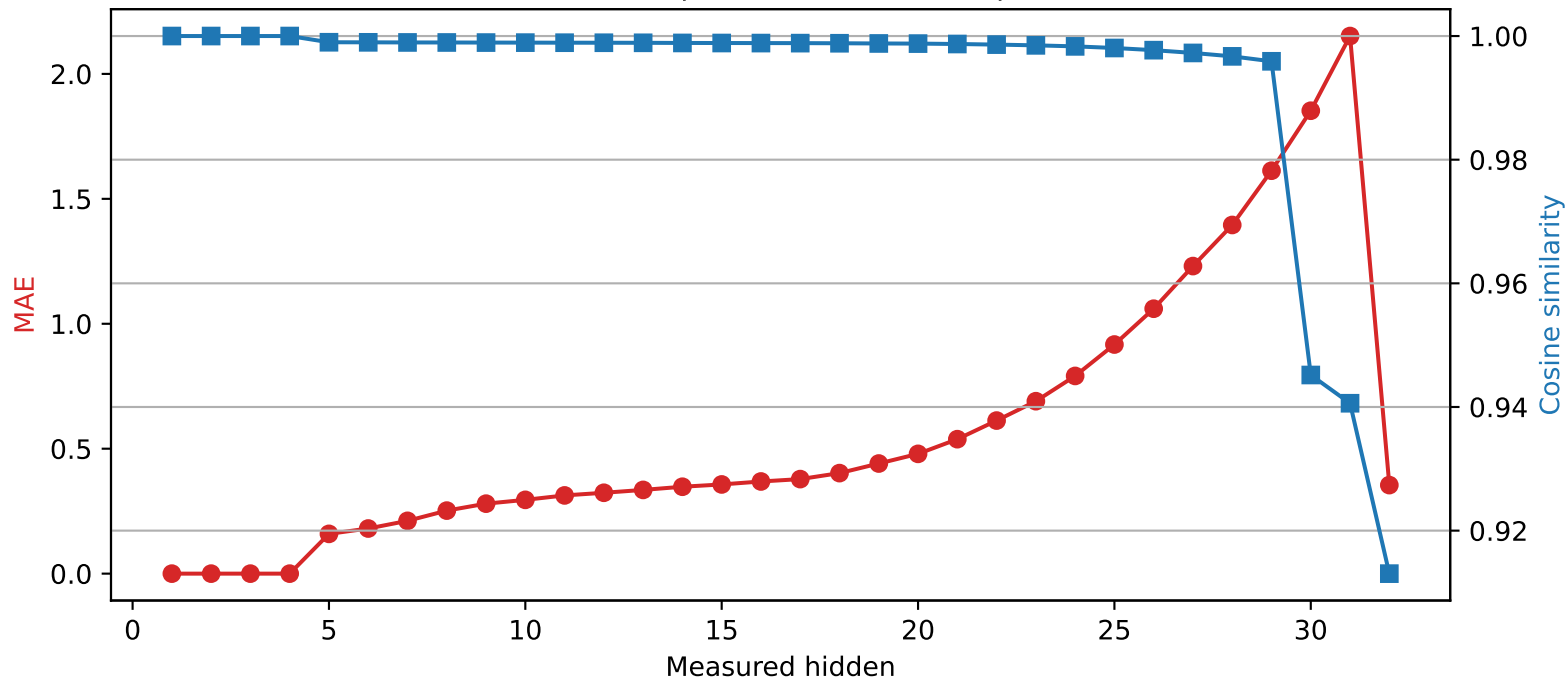
Phi-3-mini-4k-instruct | Quantized layer 4 | float32 \rightarrow int4
