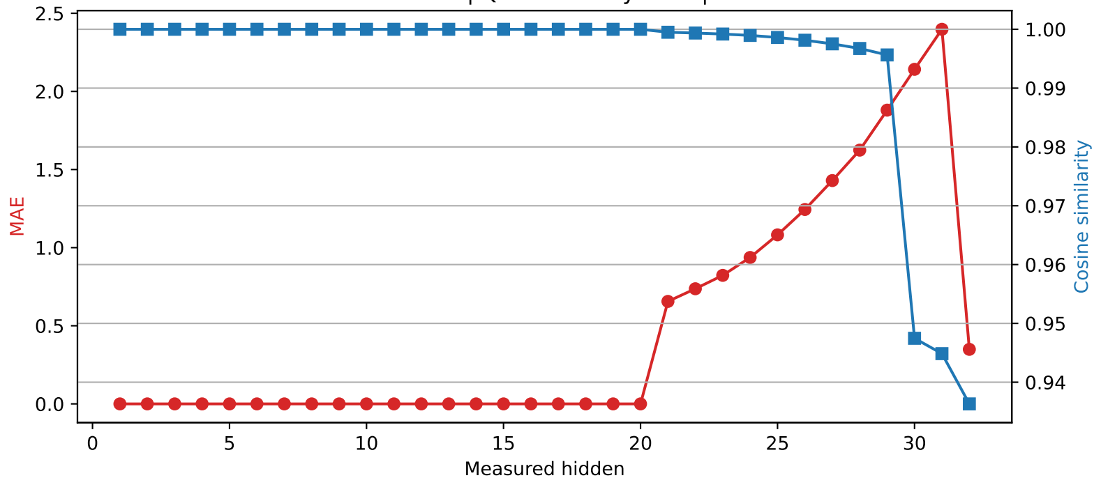
Phi-3-mini-4k-instruct | Quantized layer 20 | float32 \rightarrow int4
