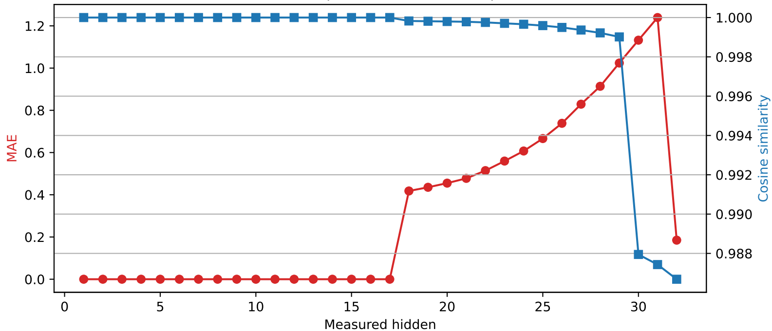
Phi-3-mini-4k-instruct | Quantized layer 17 | float32 \rightarrow int4
