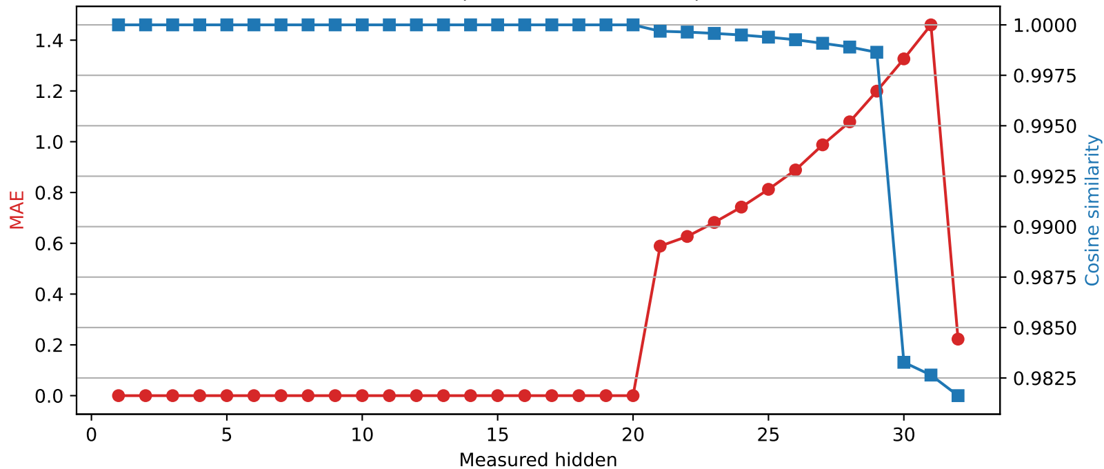
Phi-3-mini-4k-instruct | Quantized layer 20 | float32 → int4
