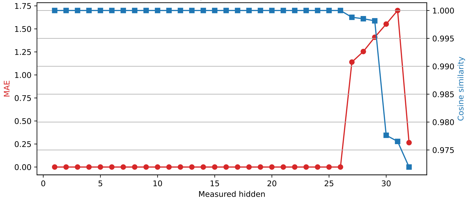
Phi-3-mini-4k-instruct | Quantized layer 26 | float32 → int4
