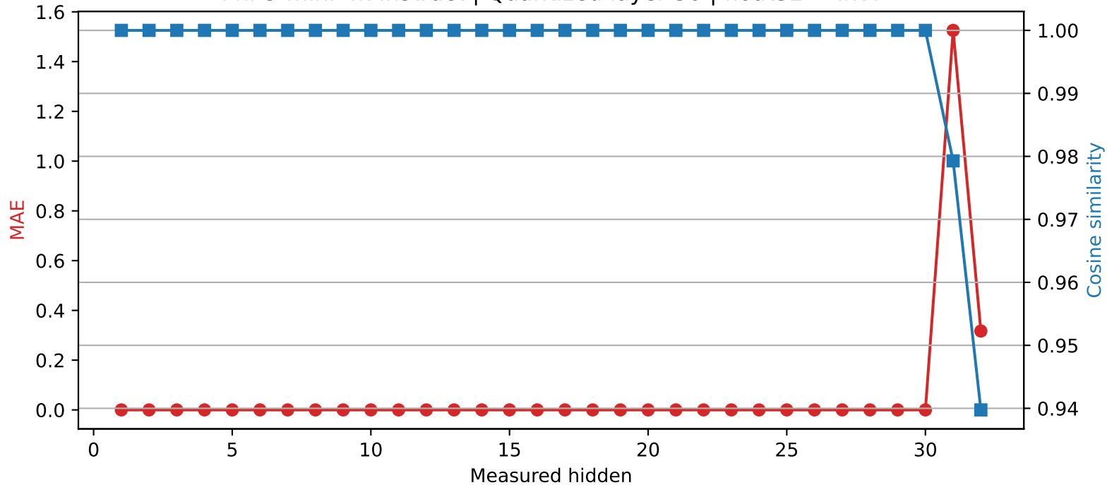
Phi-3-mini-4k-instruct | Quantized layer 30 | float32 \rightarrow int4
