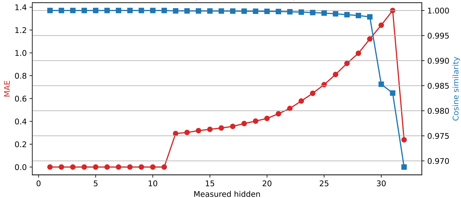
Phi-3-mini-4k-instruct | Quantized layer 11 | float32 → int4
