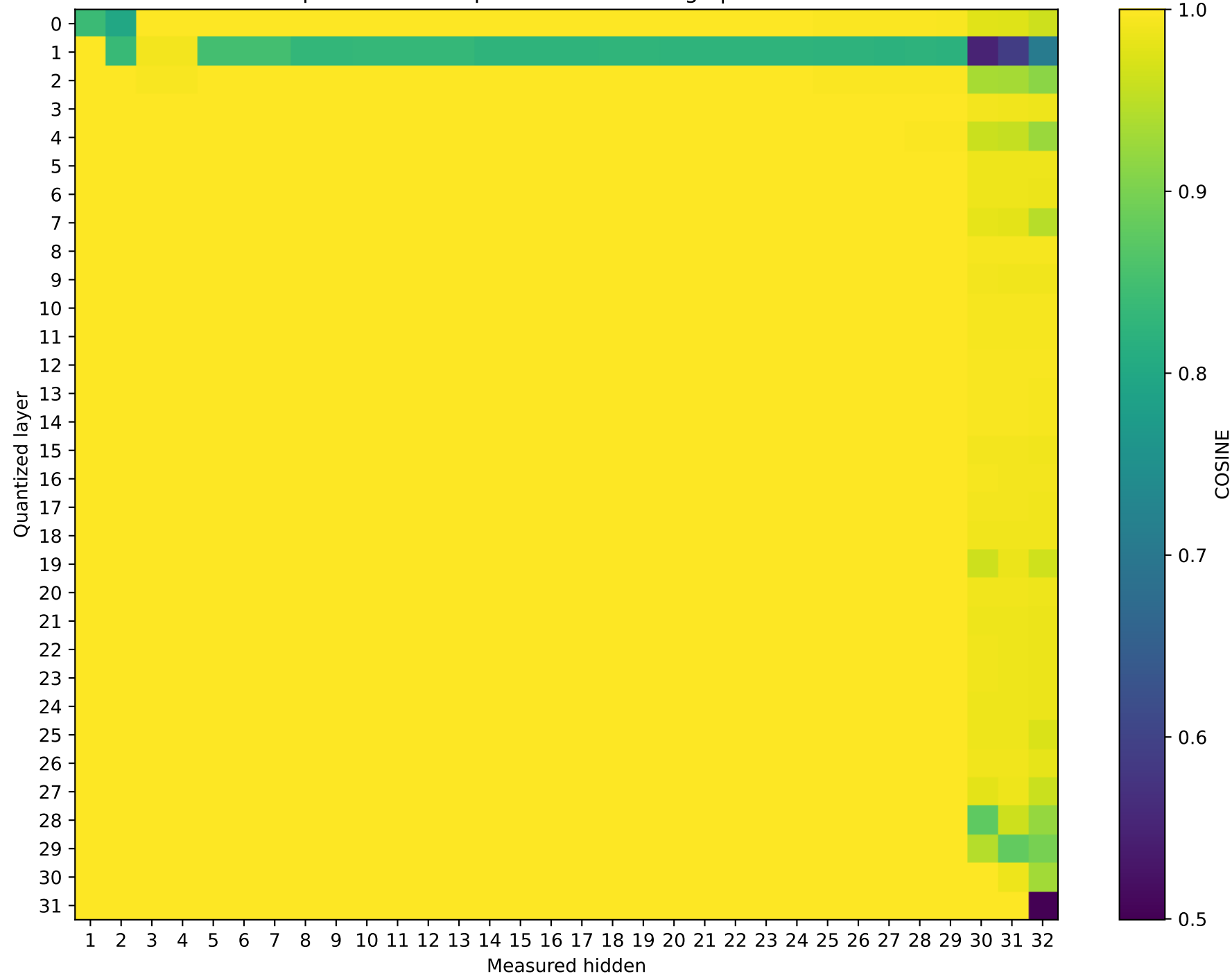
Phi-3-mini-4k-instruct Prompt 4: cos sim representation damage | float32 \rightarrow int4
