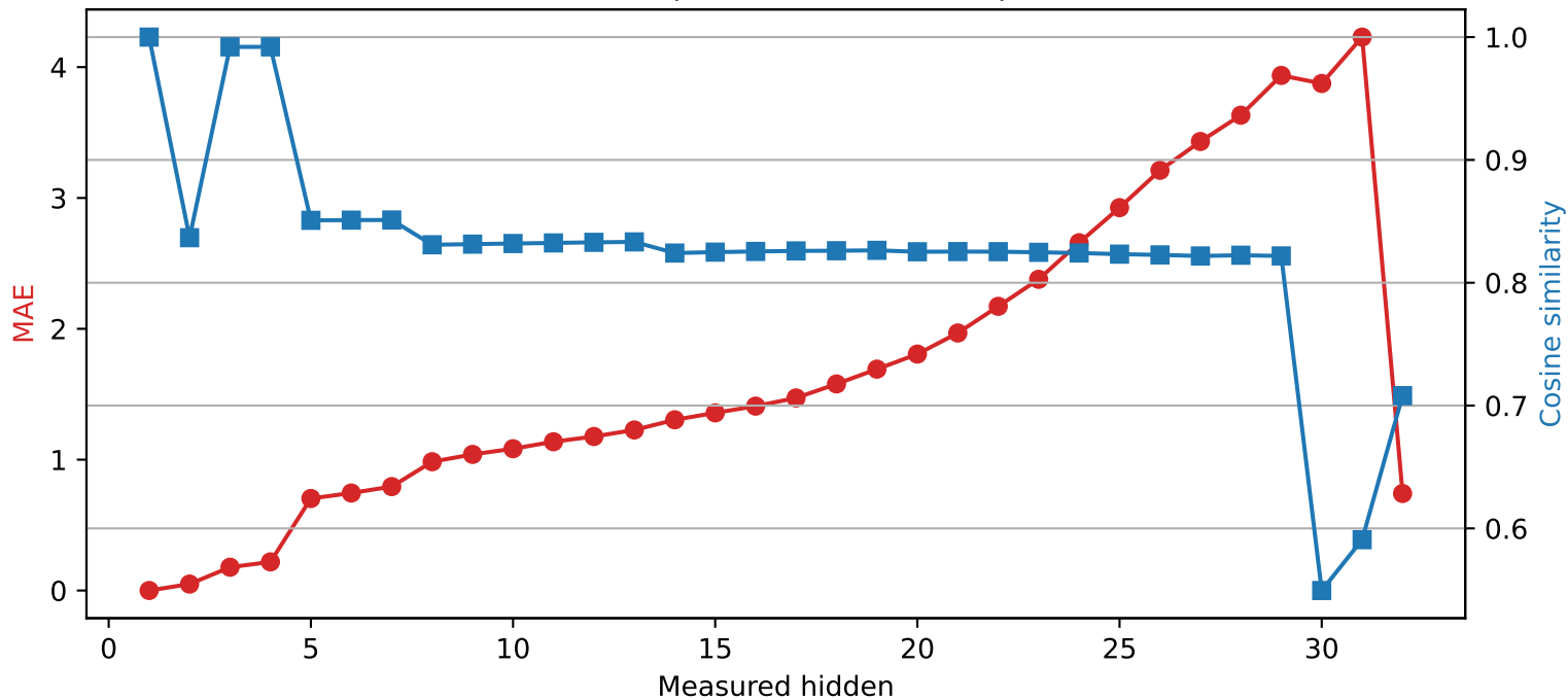
Phi-3-mini-4k-instruct | Quantized layer 1 | float32 \rightarrow int4
