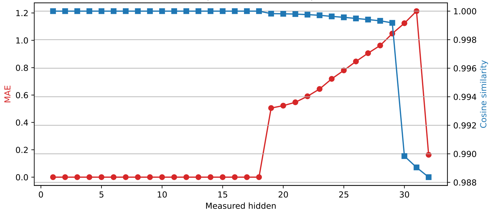
Phi-3-mini-4k-instruct | Quantized layer 18 | float32 \rightarrow int4
