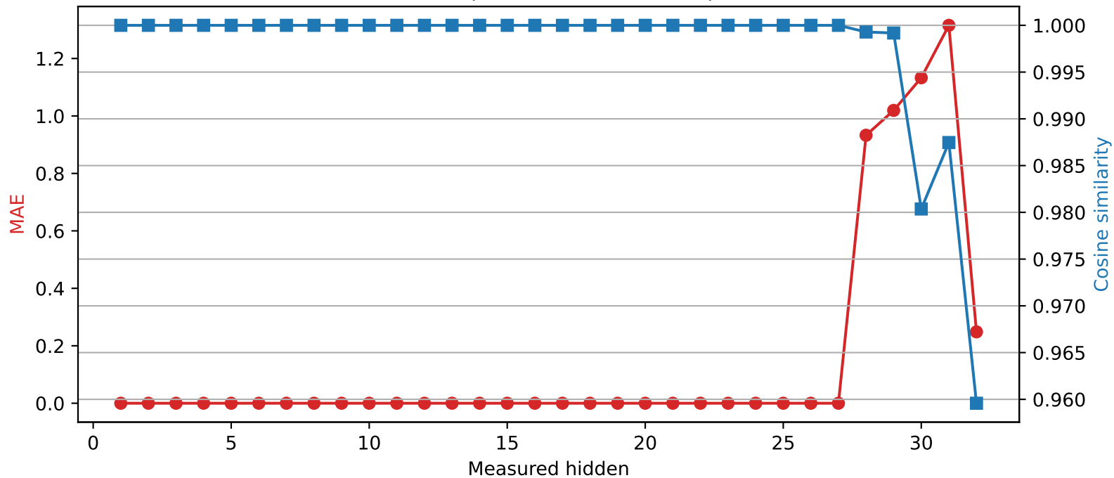
Phi-3-mini-4k-instruct | Quantized layer 27 | float32 → int4
