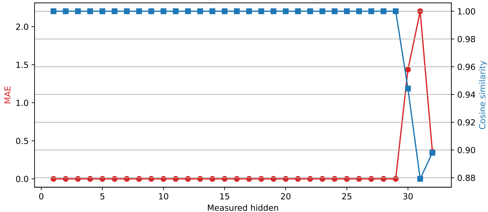
Phi-3-mini-4k-instruct | Quantized layer 29 | float32 \rightarrow int4
