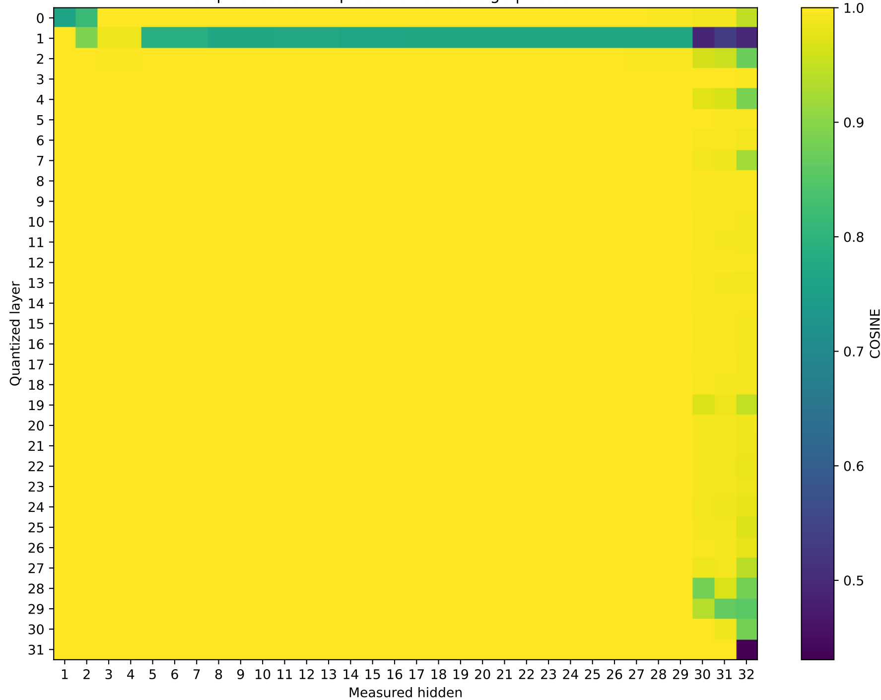
Phi-3-mini-4k-instruct Prompt 0: cos sim representation damage | float64 → int4
