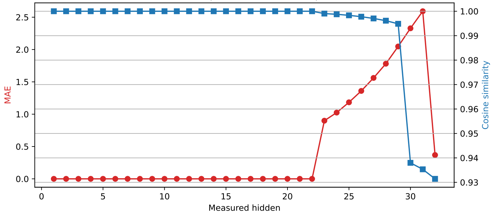
Phi-3-mini-4k-instruct | Quantized layer 22 | float64 → int4
