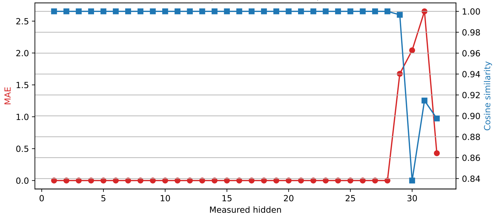
Phi-3-mini-4k-instruct | Quantized layer 28 | float64 → int4
